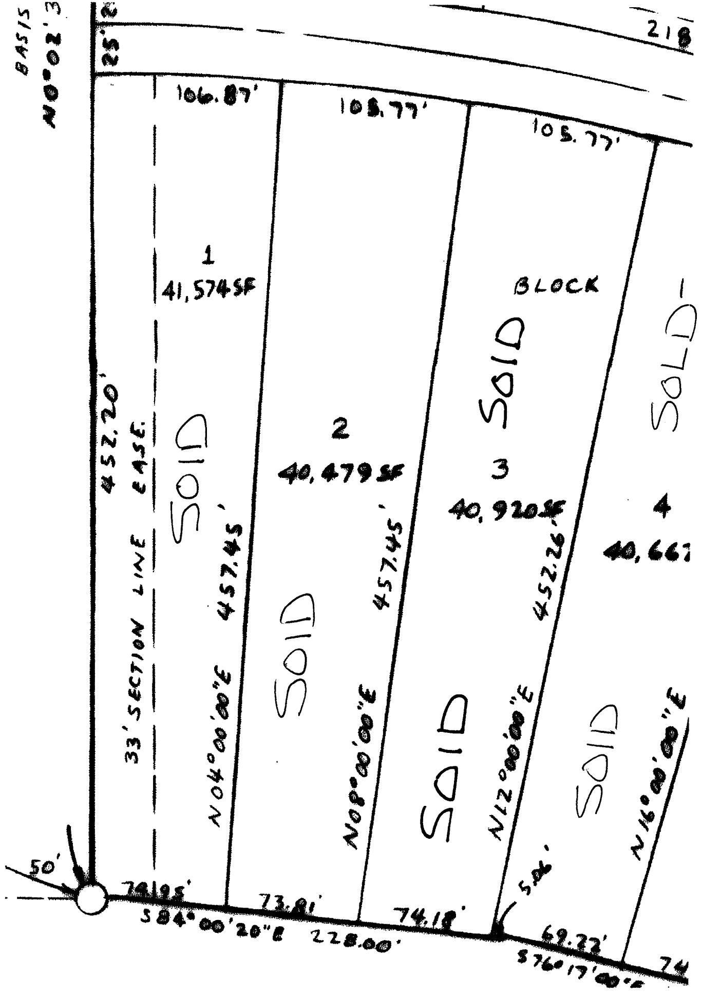
Lot 1, 2 and 3 Block 1 Lakeridge Subdivision
